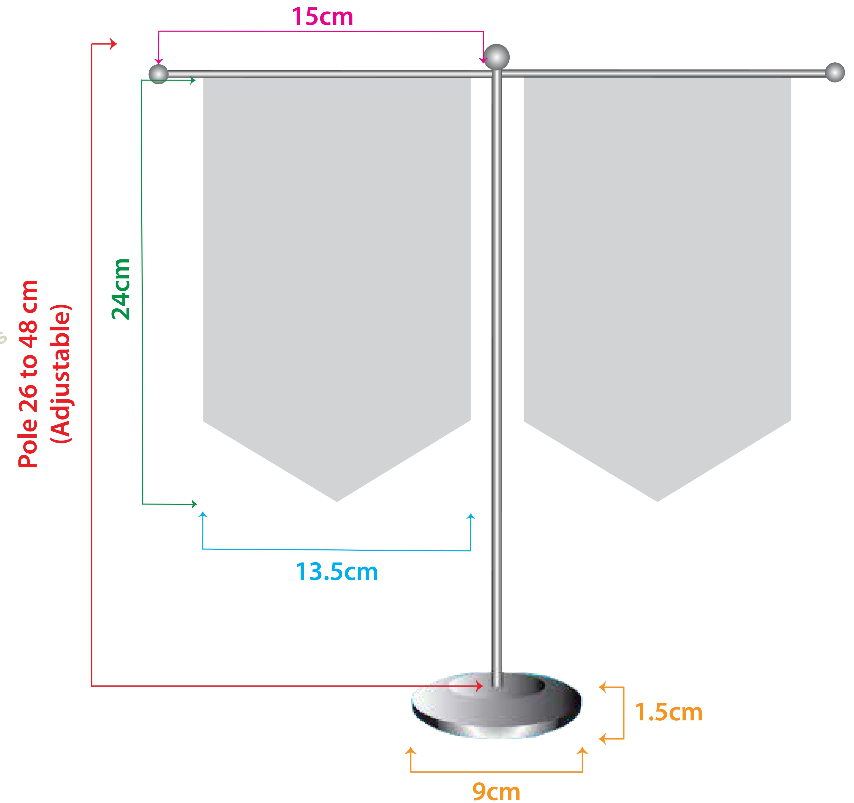
T Shape V Cut
